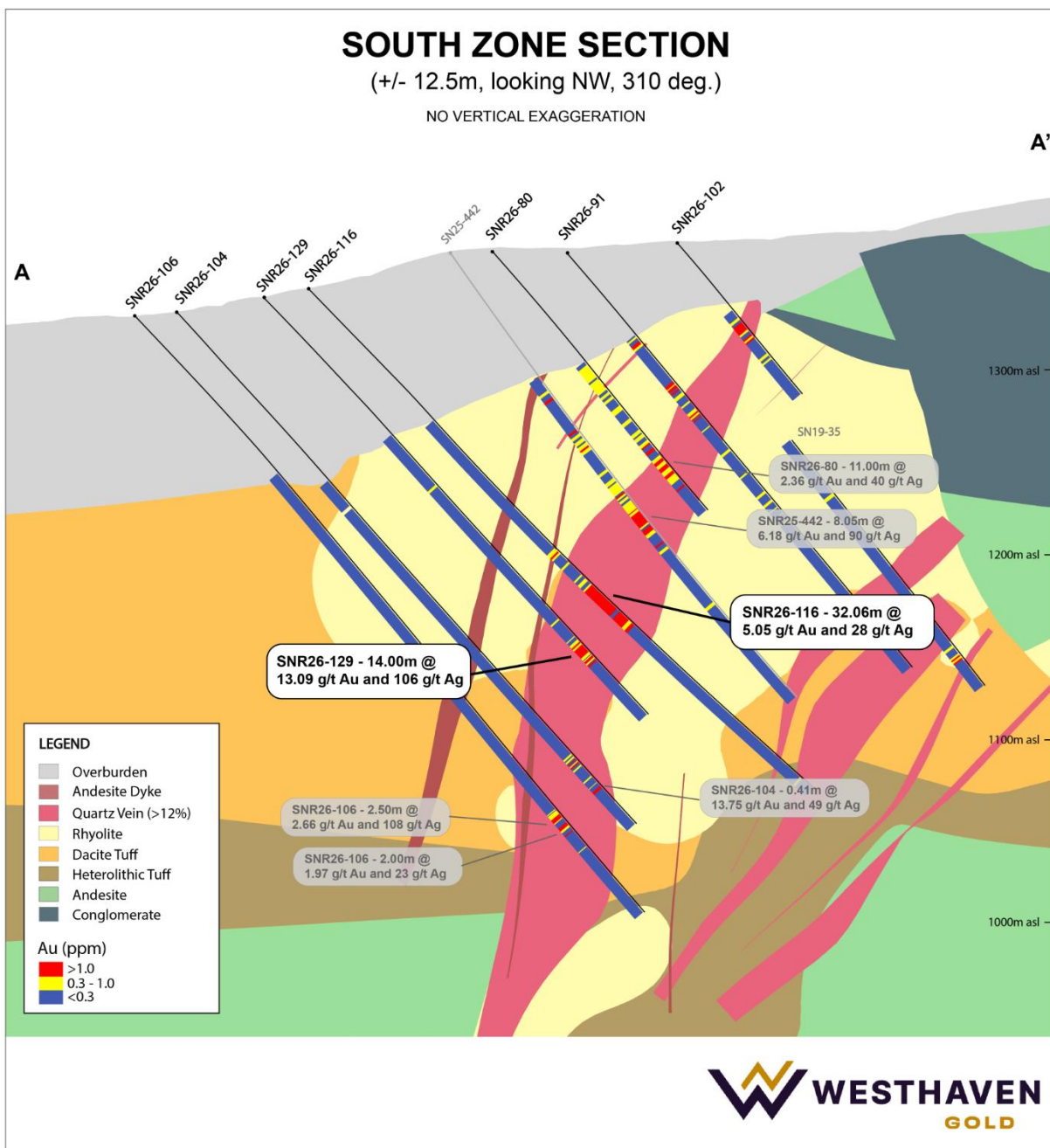
Figure 2 – South Zone Cross Section A-A'
