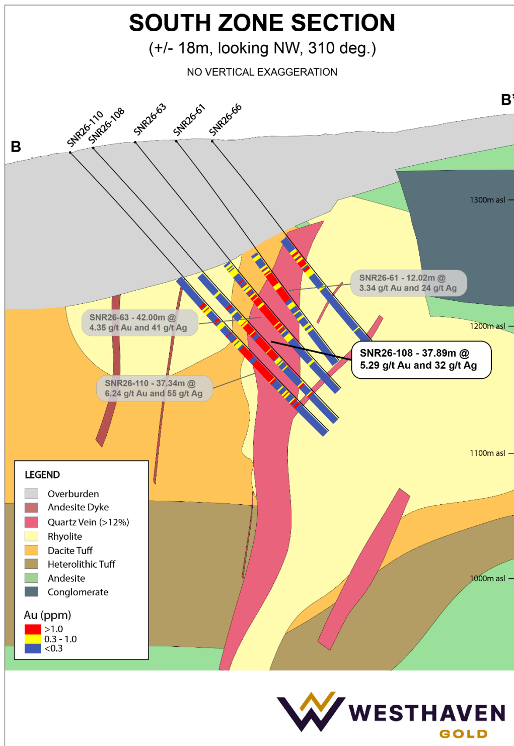
Figure 3 – South Zone Cross Section B-B'
